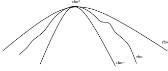
FIGURE 5. Functions in the comparison lemma.
